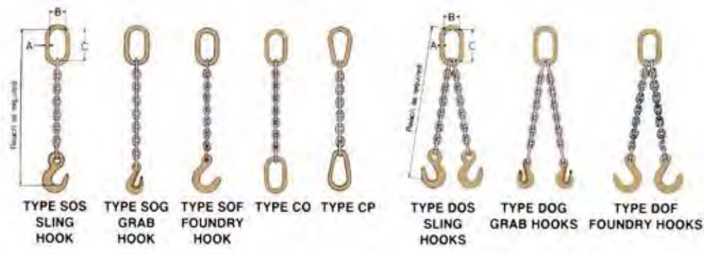
Figure 4-24 Assorted Chain slings
