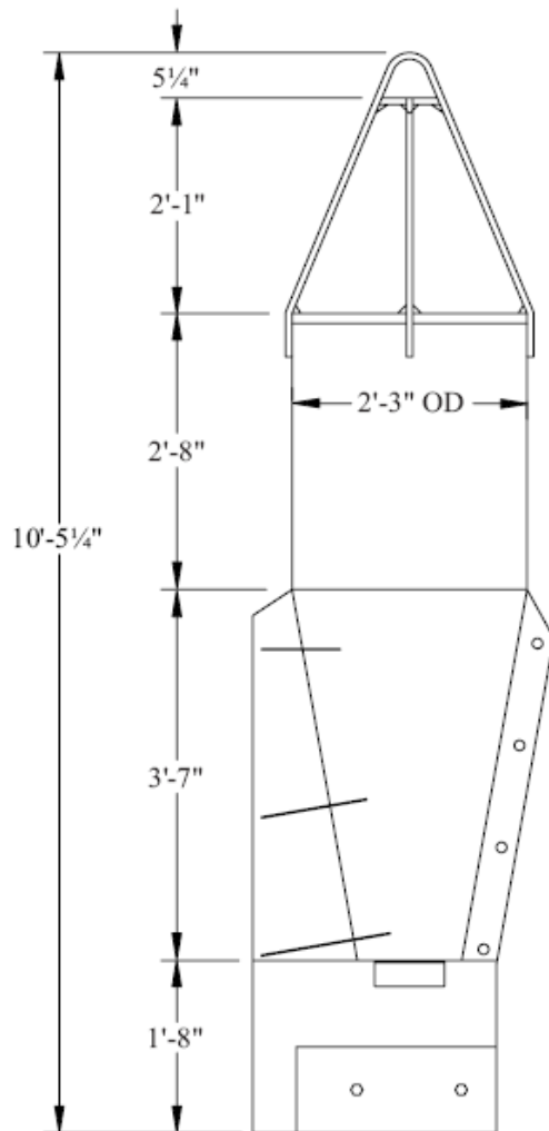
11-1 4th Class Buoy (4NR)
