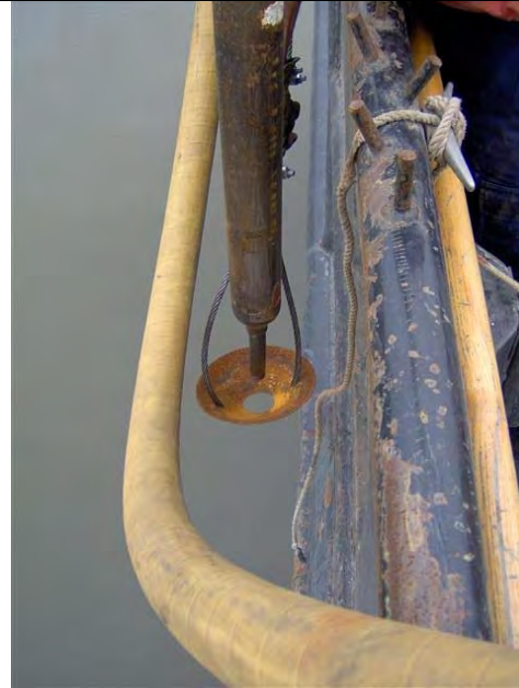
Figure 11-6 Jet Pipe Over the Side
